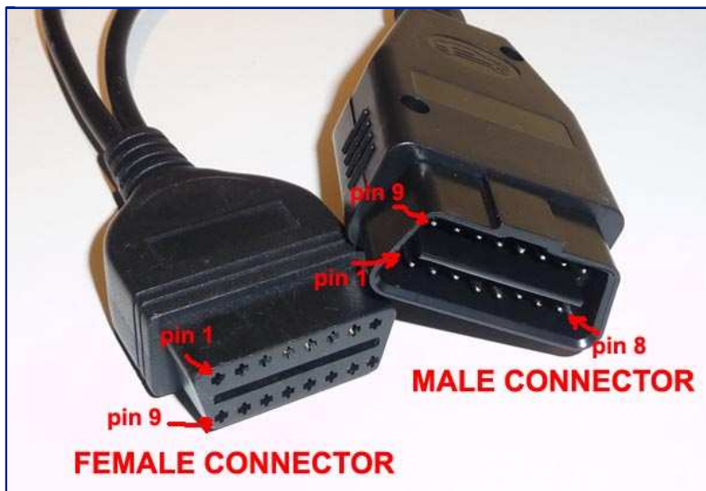
The picture above shows the actual pin numbering of the connectors.
