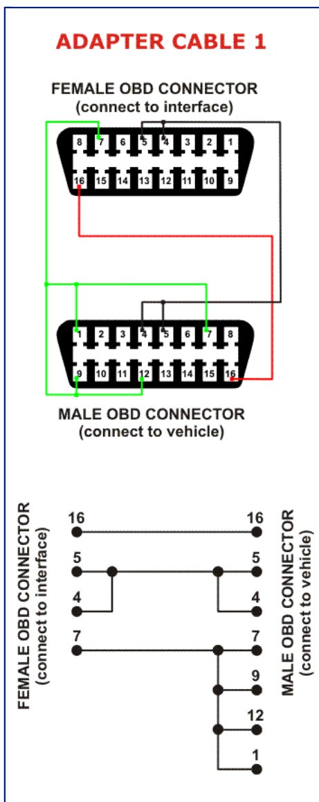
The picture above shows the actual pin numbering of the connectors.
